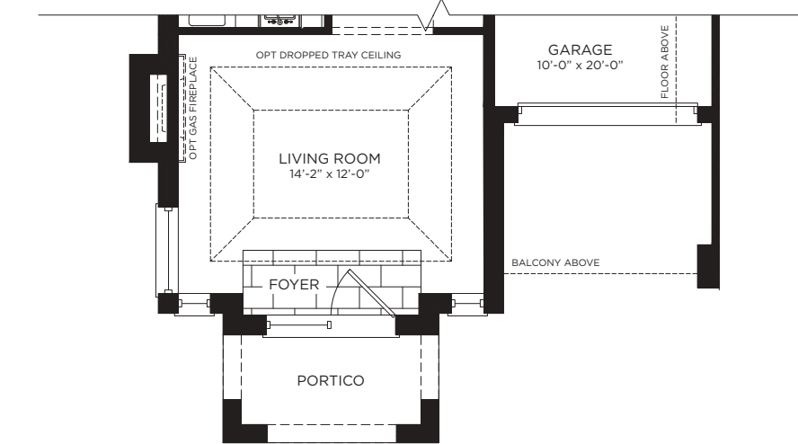
Part Ground Floor - Elevation B
