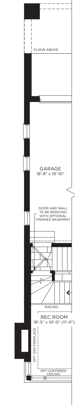
Partial Ground Floor Corner Unit
