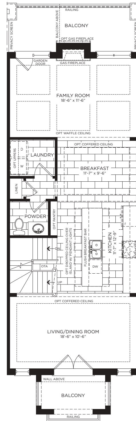
Main Floor
