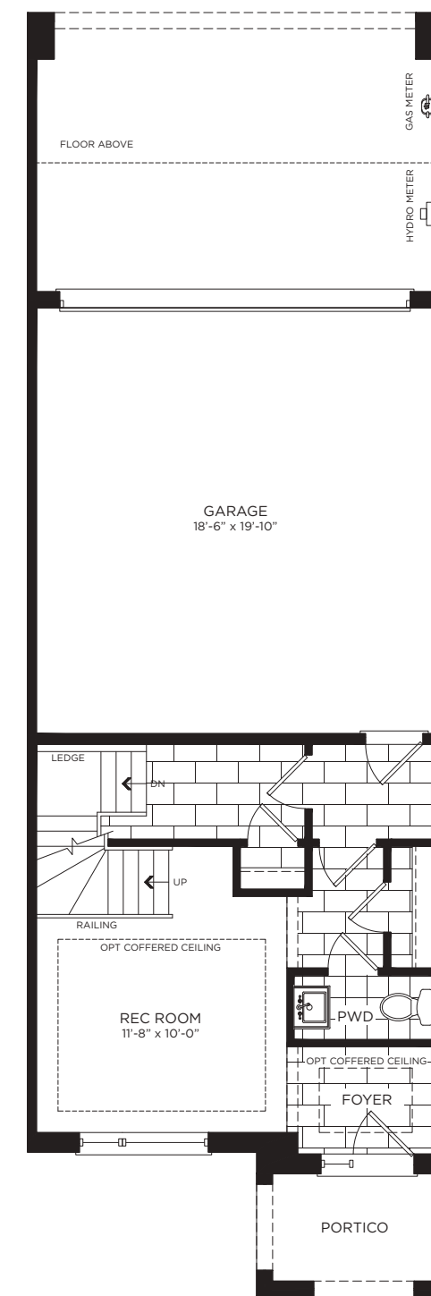
Opt. Ground Floor
