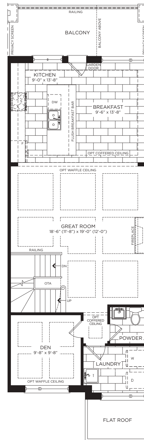
Main Floor
