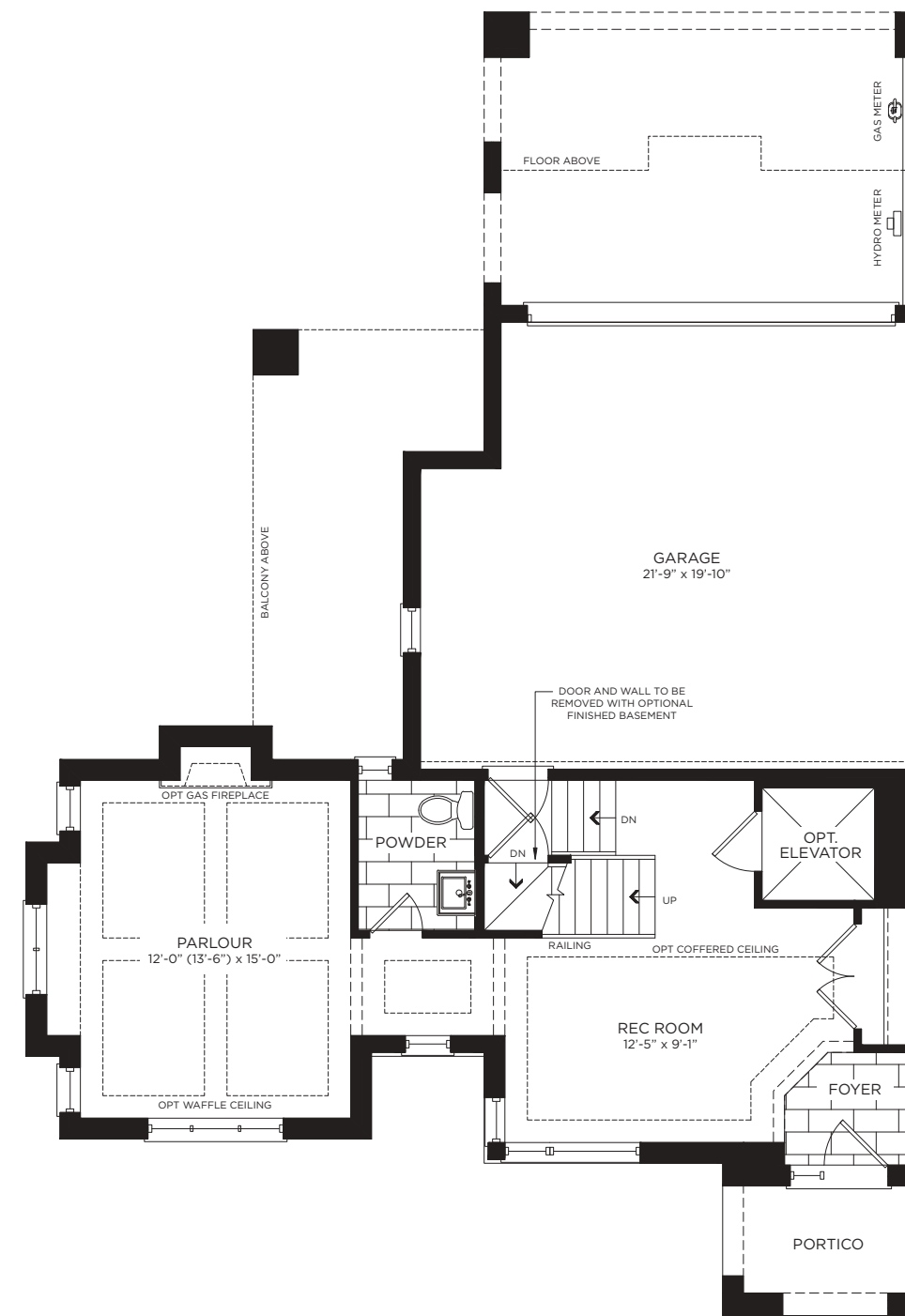
Ground Floor
