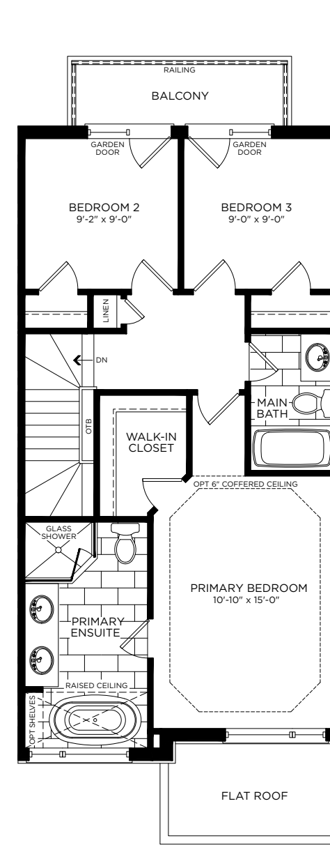
Upper Floor
